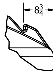
DETAIL A SCALE 0.06 : 1
